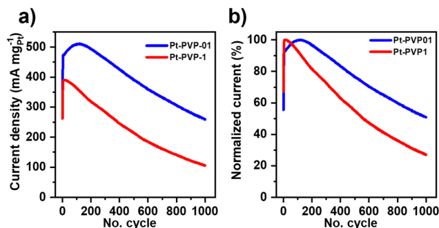
Fig. 4 Accelerated stability test (ADT) of Pt-PVP-01 and Pt-PVP-1 in 0.5 M \text{H}_2\text{SO}_4 + 1.0 M MeOH solution at 50 \text{mV s}^{-1} . (a) MA value at the i_r , (b) normalized data to the highest value.
