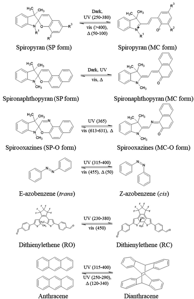
Fig. 1 Photo-switchable molecules used in the guest@MOF systems with the isomerization wavelengths given in nm and temperature in ^{\circ}\text{C} .
