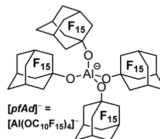
Fig. 1 Illustration of the novel WCA [pfAd]^- = [Al(OC_{10}F_{15})_4]^- .
