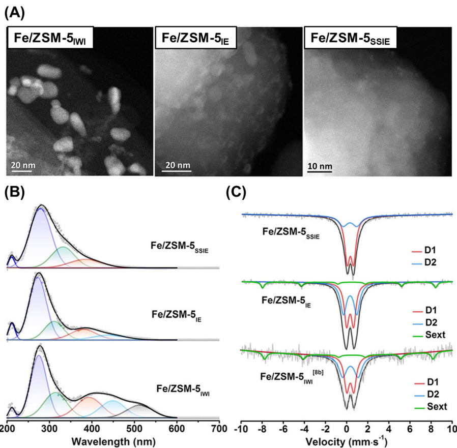
Fig. 15 (A) STEM images, (B) UV-vis spectra, and (C) ^{57}\text{Fe} Mössbauer spectra of Fe/ZSM-5s. Reprinted from ref. 65 with permission from John Wiley and Sons, copyright 2021.
