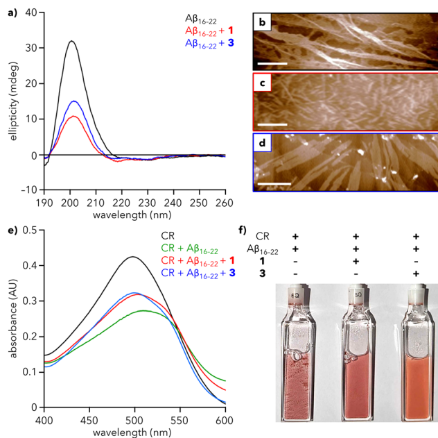
Fig. 4 Effect of dendrons on A \beta_{16-22} fibrillation. (a) CD spectra of A \beta_{16-22} alone (200 \mu M) and with 1 and 3 (30 \mu M) in water at 25 ^{\circ} C. (b)–(d) AFM images of (b) A \beta_{16-22} alone and with (c) 1 and (d) 3 . Scale bars = 500 nm. (e) UV-vis spectra of Congo red (CR) alone (100 \mu M), with A \beta_{16-22} (200 \mu M), and with 1 and 3 (30 \mu M) in water at 25 ^{\circ} C after 1 h. Spectra at 0 h are provided in Fig. S12 (ESI ^{\dagger} ). (f) Photograph of the samples from (e) after 26 h. Precipitate formation is most visible in the cuvettes containing CR + A \beta_{16-22} .
