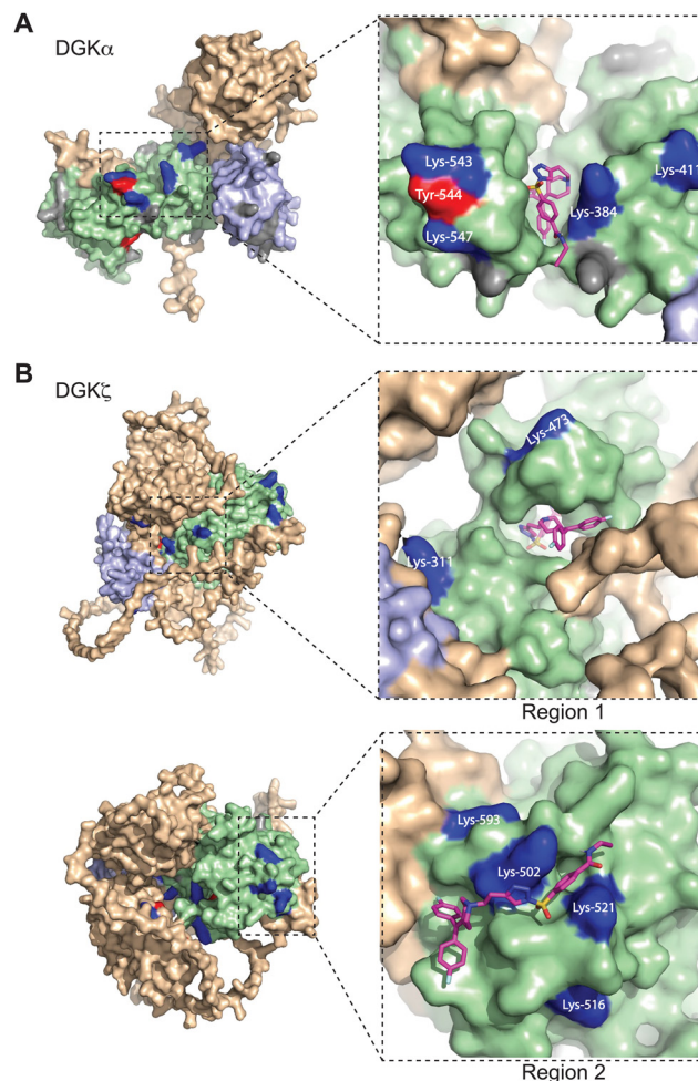
Fig. 3 Covalent binding to predicted pockets of DGK \alpha and DGK \zeta . Binding sites detected from TH211 treatments of recombinant DGK overexpressed-HEK293T cells and quantitative chemical proteomics are mapped onto AlphaFold structures (DGK \alpha : AF-P23743-F1; DGK \zeta : AF-Q13574-F1). Cells were treated with TH211 (50 \mu M) for 2 h at 37 °C. The covalent binding profiles of DGK \alpha and DGK \zeta are shown here. The remaining DGK protein AlphaFold structures can be found in Fig. S3 (ESI†). (A) DGK \alpha with inset showing expanded region of TH211 docked on Lys-384 in the predicted binding pocket. (B) DGK \zeta with inset showing expanded region with TH211 docked on Lys-473. A second predicted binding pocket of DGK \zeta with inset showing expanded region of TH211 docked on Lys-502. C1A and C1B domains are shaded light blue, and the catalytic domain (DAGKc and DAGKa regions) is shaded in light green. Probe modified Lys and Tyr are shown in dark blue and red, respectively. Lys and Tyr residues confidently predicted by AlphaFold ("Confident" and "Very Confident" predictions, pLDDT > 70) but not modified by our probe are shown in gray. Lys and Tyr residues predicted less confidently ("Low" and "Very Low" predictions, pLDDT < 70) are not highlighted and were not included in the analysis. All data shown are representative of n = 3 biologically independent experiments. Predicted structures were visualized using PyMOL (Version 2.6; https://pymol.org ).
