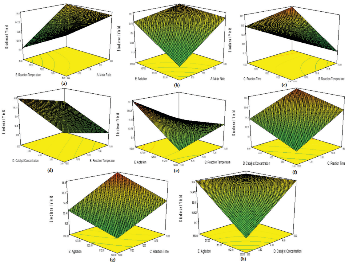
Fig. 9 (a) 3D surface plot of the interactive effects of the molar ratio and reaction temperature on % biodiesel. (b) 3D surface plot of the interactive effects of the molar ratio and agitation on % biodiesel. (c) 3D surface plot of the interactive effects of reaction time and reaction temperature on % biodiesel. (d) 3D surface plot of the interactive effects of catalyst concentration and reaction temperature on % biodiesel. (e) 3D surface plot of the interactive effects of agitation speed and reaction temperature on % biodiesel. (f) 3D surface plot of the interactive effects of catalyst concentration and reaction time on % biodiesel. (g) 3D surface plot of the interactive effects of agitation speed and reaction time on % biodiesel. (h) 3D surface plot of the interactive effects of agitation speed and catalyst concentration on % biodiesel.
