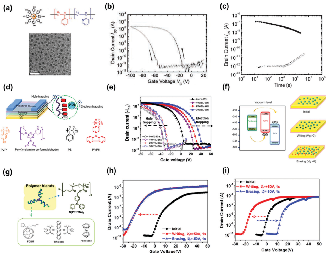
Fig. 9 (a) Schematic representation of Au NPs with multiple H-bond-donating groups, chemical structure of PS-P2VP, and TEM image of Au NPs. (b) Dual sweeping I-V curve of the device using electret comprising 40% Au NPs. (c) Retention time test of the memory devices. Reproduced with permission. 62 Copyright 2012, American Chemical Society. (d) Schematic configuration of the OFET memory device and the chemical structure of the polymer matrix. (e) Transfer characteristics after electrical writing and erasing of the memory device using PVPK/ZnO as nano-floating gates. (f) Mechanisms and energy band diagrams under positive and negative bias. Reproduced with permission. 63 Copyright 2015, Springer Nature. (g) Chemical structure of n -polymer dielectric of N(PTPMA) 3 and organic materials of PCBM, TIPS-pen, and ferrocene. Transfer characteristics after electrical writing and erasing of the memory device with (h) N(PTPMA) 3 and (i) 5 wt% PCBM:N(PTPMA) 3 as electrets. Reproduced with permission. 64 Copyright 2014, American Chemical Society.
