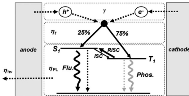
Fig. 1 Schematic view of the electroluminescence mechanism: carrier injection, transport, recombination; and radiative decay processes. The thermally activated delayed fluorescence (TADF) process is highlighted ( \gamma : ratio of holes and electrons in carrier injection, transport, and recombination processes; \eta_r : singlet and triplet exciton formation ratio; \eta_{PL} : photoluminescence efficiency; \eta_{hv} : light out-coupling efficiency; ISC: intersystem crossing; and RISC: reverse intersystem crossing). Reprinted (adapted) with permission. 60 Copyright © 2009 WILEY-VCH Verlag GmbH & Co. KGaA, Weinheim.
