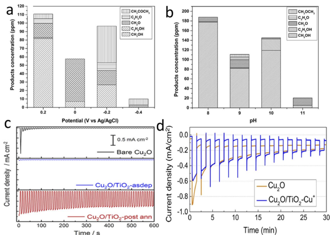
Fig. 7 The product distributions after 2 h of the PEC \text{CO}_2\text{RR} (a) at different potentials at pH 9 and (b) at different pH levels at +0.2 \text{ V}_{\text{Ag/AgCl}} . Current density vs. time plots clearly showing that the data from the annealed \text{TiO}_2 coated photoelectrode in the 3 rd row of (c) are much more stable than those shown in (d), (a) and (b) are reproduced with permission from de Brito et al. , 115 Copyright 2015, Elsevier Ltd. (c) Kang et al. , 117 Copyright 2018, American Chemical Society; (d) is from Lee et al. , 116 Copyright 2018, Elsevier Ltd.
