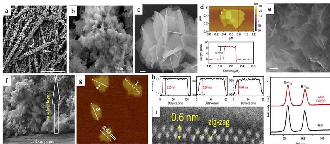
Fig. 16 (a), (b) SEM images of Bi NSs on carbon fiber. (c) An SEM image of BiOI NSs; 200 nm scale bar. (d) An AFM image and the corresponding height profile. (e) An SEM image of topotactically reduced Bi NS; 200 nm scale bar. (f) An SEM image of a bismuthene catalyst layer on a carbon paper electrode; 1.0 \mu\text{m} scale bar. (g) An AFM image and (h) corresponding height profiles for the three bismuthene NSs marked in (g). (i) A lateral HAADF-STEM image of a bismuthene NS, showing a zig-zag structured layer with single-atom thickness. (j) High-resolution Bi 4f XPS spectra before and after 75 h of the \text{CO}_2\text{RR} process at -0.58 V_{\text{RHE}} . (a), (b) are reproduced with permission from Su et al. , 211 Copyright 2018, John Wiley and Sons, (c)–(e) from Han et al. , 212 Copyright 2018, Springer Nature Limited, (f)–(j) from Yang et al. , 215 Copyright 2020, Springer Nature Limited.
