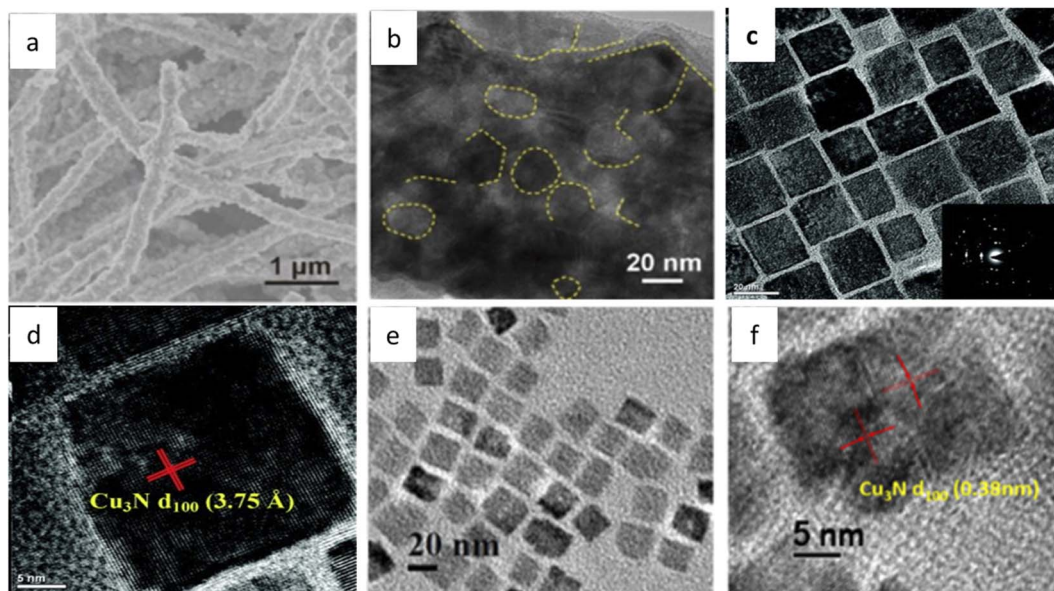
Fig. 13 (a) An SEM image of a \text{Ni}_3\text{N} -derived Cu nanowire. (b) A TEM image showing grain boundaries. (c) and (d) TEM images of \text{Cu}_3\text{N} NCs used in a fuel cell. (e) and (f) TEM images of \text{Cu}_3\text{N} NCs used in an electrocatalysis study. (a) and (b) Reproduced with permission from Mi et al. , 187 Copyright 2019, John Wiley and Sons, (c) and (d) from Wu et al. , 189 Copyright 2011, American Chemical Society and (e), (f) from Yin et al. , 188 Copyright 2019, American Chemical Society.
