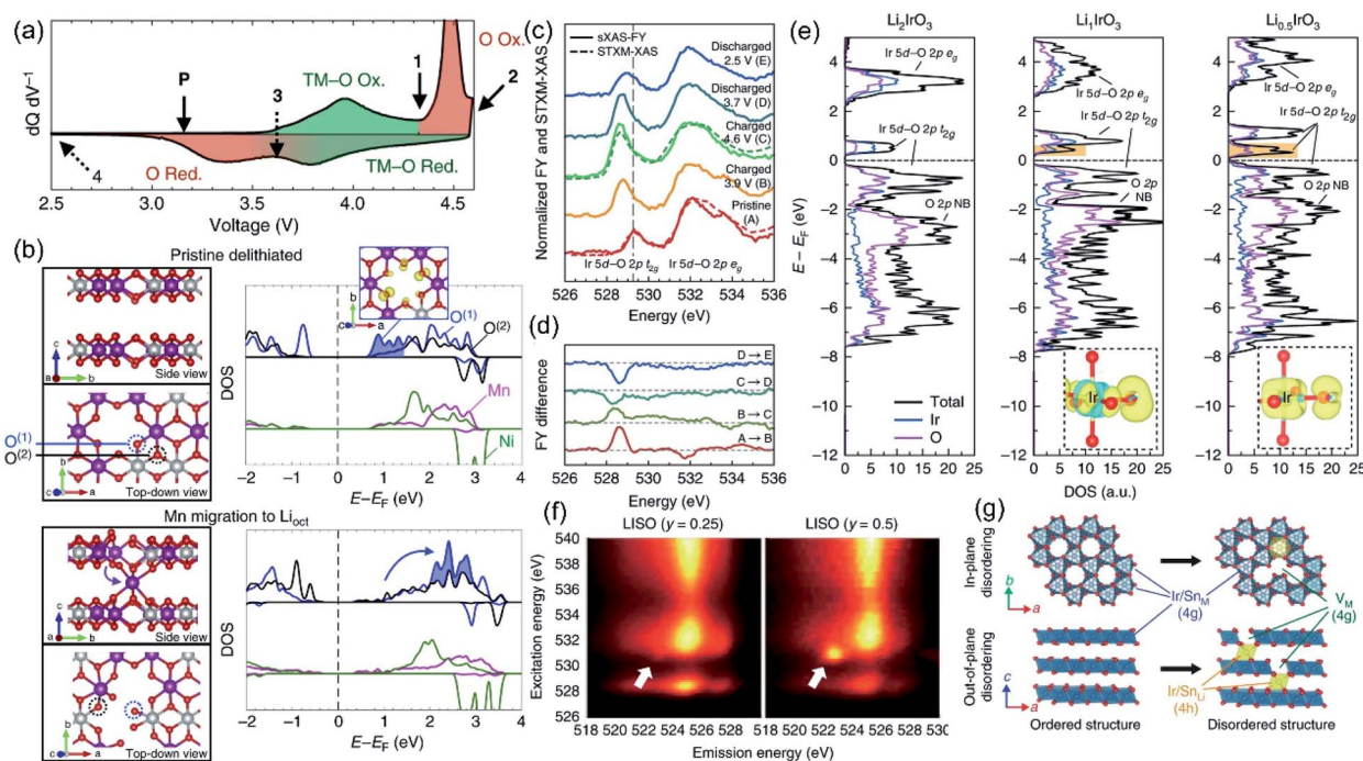
Fig. 6 (a) dQ/dV of the first cycle showing the voltages at 4.35 V (1), 4.60 V (2), 3.65 V (3), and 2.00 V (4). Regions of the dQ/dV are shaded to show the hysteresis in the O redox relative to the TM–O redox. (b) pDOS for the TMs and the two-coordinate ( \text{O}^{(1)} , blue) and three-coordinate ( \text{O}^{(2)} , black) oxygen environments in the pristine delithiated state (top), and after Mn (middle) and Ni (bottom) migration into octahedral sites in the Li layer. The integrated charge density for the lowest unoccupied states in the pristine delithiated structure (blue shaded area of the pristine DOS) is shown in the top right inset. Schematics of each supercell used to generate the pDOS are shown to the left, with the plotted \text{O}^{(1)} and \text{O}^{(2)} oxygen environments circled. Reproduced with permission from ref. 9. Copyright 2017, Springer Nature. (c) sXAS-FY spectra and STXM-XAS of the O K edge of \text{Li}_{2-x}\text{IrO}_3 at various voltages throughout the first cycle. (d) Difference plot of sXAS obtained from (c) showing the intensity evolution of Ir 5d–O 2p t_{2g} and e_g peaks. (e) Ir- and O-projected density of states of \text{Li}_2\text{IrO}_3 , \text{Li}_1\text{IrO}_3 and \text{Li}_{0.5}\text{IrO}_3 calculated from first principles. Yellow and blue show negative and positive changes in charge density, respectively. Li ions are omitted for clarity. (f) O K-edge RIXS maps of LISO25 and LISO50 charged to 4.60 V showing a localized RIXS feature at 530.7 eV excitation energy and 522.8 eV emission energy. (g) In-plane and out-of-plane disorder quantified by iterative XRD Rietveld refinement. Reproduced with permission from ref. 27. Copyright 2019, Springer Nature.
