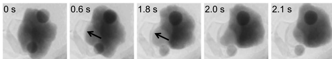
Fig. 16 Still images from in situ ETEM footage of an iron-rich particle moving through a carbon matrix. Arrows show the layers of graphite forming on the trailing edge of the catalyst. Images modified with permission from ref. 147.
