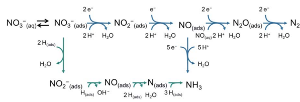
Fig. 9 The electron and adsorbed hydrogen mediated direct electrocatalytic routes for the \text{NO}_3\text{RR} . Reproduced with permission from ref. 125. Copyright 2021 Elsevier.
