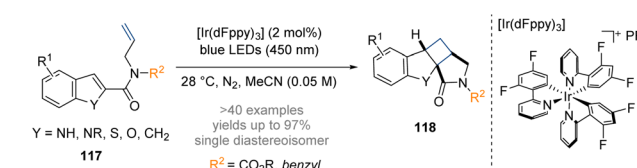
Scheme 34 Dearomative photoredox catalysed intramolecular [2 + 2] cycloaddition of indoles. 40
