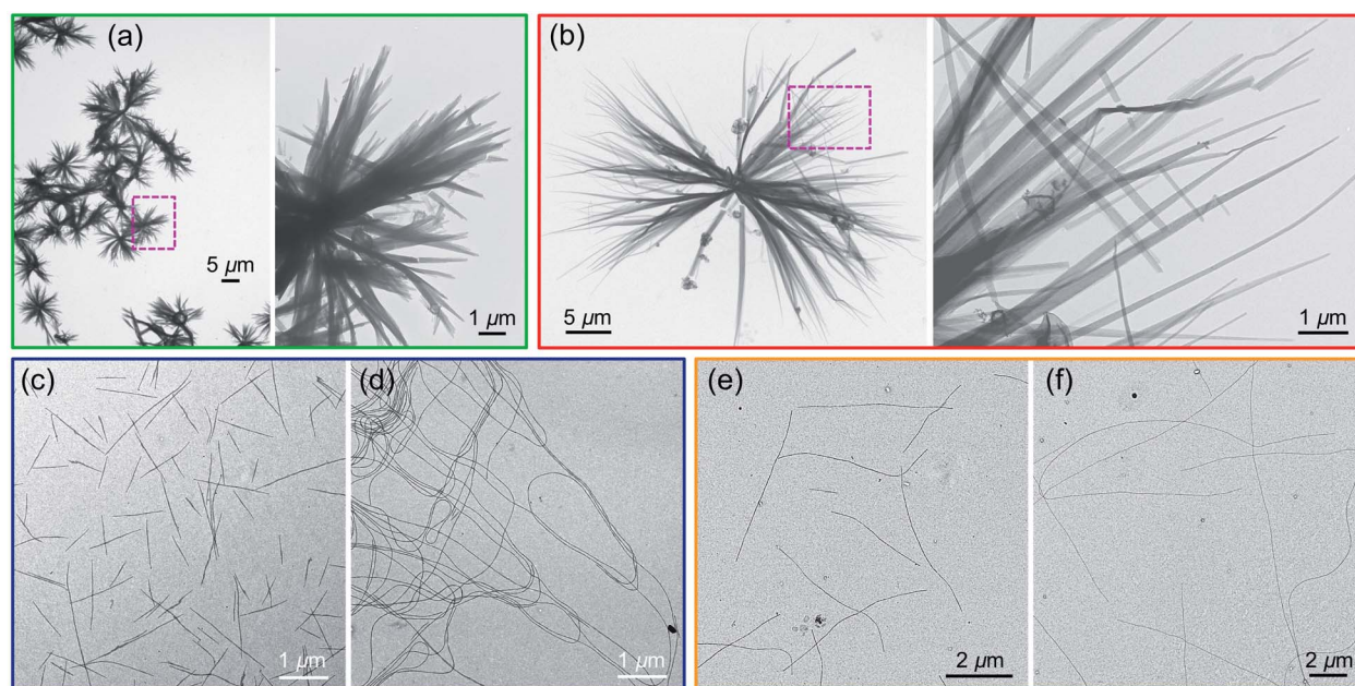
Fig. 2 TEM images of structures formed by homopolymer PFS 45 through (a) quick cooling and (b) slow cooling process after heating in decane (0.05 \text{mg mL}^{-1} , 1 mL) at 140 °C for 30 min and then cooling to RT. TEM images of micelles formed by PFS 25 - b -P2VP 330 through (c) quick cooling and (d) slow cooling process after heating in 2-propanol (0.5 \text{mg mL}^{-1} , 1 mL) at 80 °C for 30 min and cooling to RT. TEM images of micelles formed by PFS 35 - b -PI 273 through (e) quick cooling and (f) slow cooling process after heating in decane (0.5 \text{mg mL}^{-1} , 1 mL) at 80 °C for 30 min and cooling to RT.
