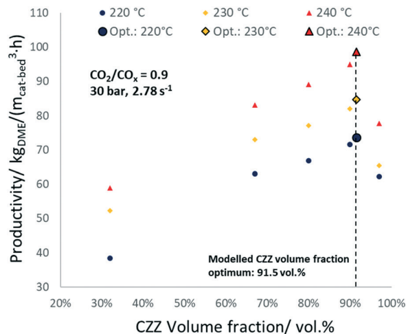
Fig. 6 Comparison of the experimental DME productivity in the run-in period and the model-optimized CZZ/ FER volume ratio of 91.5/8.5 at CO_2/CO_x = 0.9 , 30 bar, 2.78 \text{ s}^{-1} and three different temperatures.
