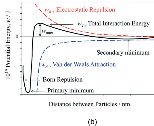
Fig. 10 (a) Schematic pH effect on surface charge and hence zeta potential on metal oxide particles. (b) Schematic effect of inter-particle separation on electrostatic repulsion ( w_R ), van der Waals attraction ( w_A ), and total ( w_T = w_R + w_A ) interaction potentials.
