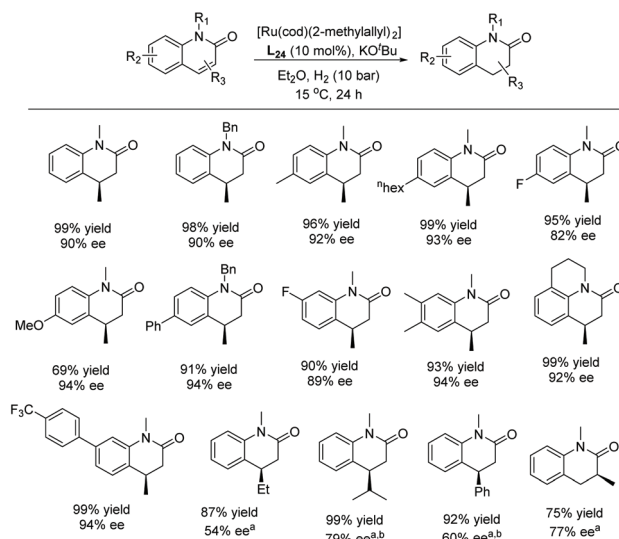
Scheme 49 EH of substituted 2-quinolones using Ru-NHC catalyst. [Ru(cod)(2-methylallyl)_2] (5 mol%), KOtBu (12.5 mol%), Et_2O (1 mL). a Hexane (1 mL) and H_2 (70 bar). b 30\text{ }^\circ\text{C} , 20% [Ru] catalyst and H_2 (70 bar) for 48 h.
