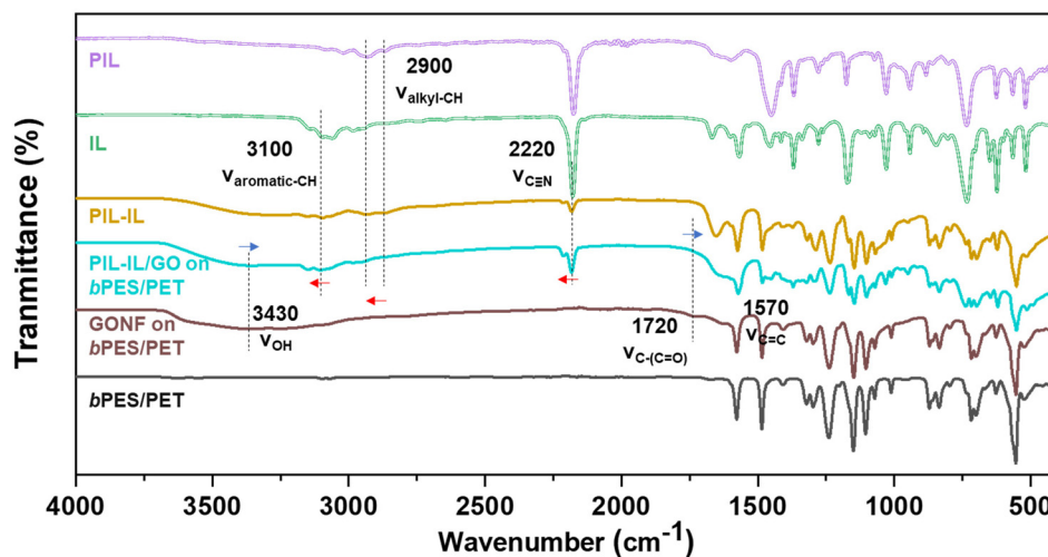
Fig. 5 FTIR spectra of PIL, IL, PIL-IL, PIL-IL/GO on b PES/PET, GONF on b PES/PET, and b PES/PET substrate. The vertical dashed lines mark the resonance peak of \nu_{\text{OH}} 3430 \text{cm}^{-1} (GONF), \nu_{\text{aromatic-CH}} 3100 \text{cm}^{-1} (IL), \nu_{\text{alkyl-CH}} 2900 \text{cm}^{-1} (PIL), \nu_{\text{C}\equiv\text{N}} 2220 \text{cm}^{-1} (PIL and IL), \nu_{\text{C}-(\text{C}=\text{O})} 1720 \text{cm}^{-1} (GONF), \nu_{\text{C}=\text{C}} 1570 \text{cm}^{-1} (GONF). The arrows indicate the red and blue shift-direction of each vibration in the PIL-IL/GO, due to molecular interactions among the constituents.
