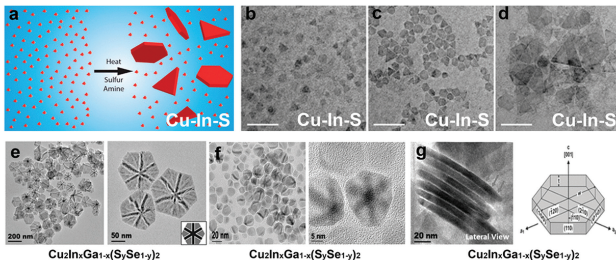
Fig. 8 (a) Schematic representation of the formation of Cu–In–S nanosheets generated via oriented attachment of CuInS 2 nanopillars, TEM image depicting the evolution of the nanosheets collected after (b) 1 min, (c) 2 min (d) 5 min; Reproduced from ref. 21 with permission from ACS, copyright 2017; (e) TEM image of the Cu 2 In x Ga 1-x (S y Se 1-y ) 2 disc with bend contours synthesised using TOPO as the coordinating solvent, (f) TEM image of the Cu 2 In x Ga 1-x (S y Se 1-y ) 2 disc with shallow bend contours synthesised using TOPO and OLA as the solvent, (g) TEM image showing lateral view of the nanodisc where the cartoon depicts the prismatic and basal planes. Reproduced from ref. 54 with permission from ACS, copyright 2018.
