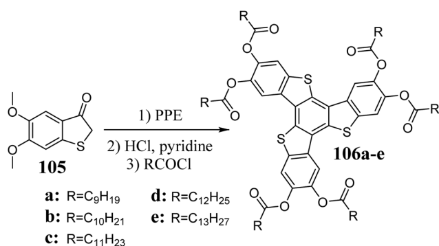
Scheme 38 Synthesis of 5,10,15-trithiatruxene ester derivatives.
