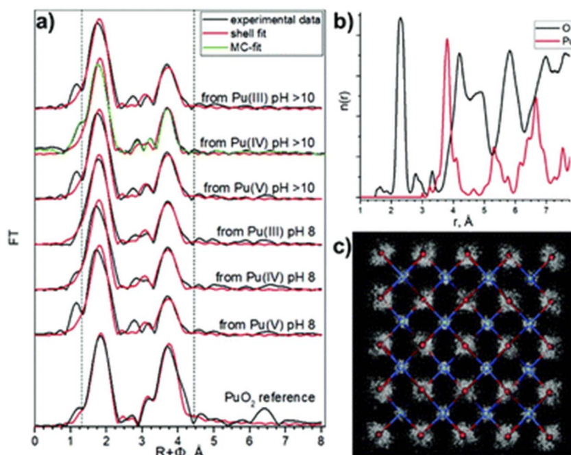
Fig. 14 (a) FT magnitude of experimental Pu L_3 EXAFS spectra (black) acquired on \text{PuO}_2 nanoparticles prepared by ammonia addition into \text{Pu(III)} – \text{Pu(V)} aqueous solutions. \chi(R) fit results obtained with one Pu–O and one Pu–Pu shell fit are represented in red and Monte-Carlo simulation fits are represented in green. The two vertical dashed lines represent the area of the shell fit. (b) Radial particle distribution function ( n(r) ) for Pu–O and Pu–Pu obtained for Monte-Carlo simulation and (c) 3D structural refinement based on bulk \text{PuO}_2 structure. Reproduced from ref. 111 with permission from the Royal Society of Chemistry, copyright 2020.
