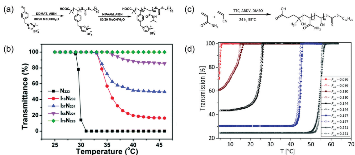
Fig. 7 Examples of effects of co-polymerization on thermoresponsive behavior. (a) Synthetic scheme of P(NIPAAm- co -[VBMI][BF 4 ]). (b) Increasing in LCST and diminishing of thermoresponsive behavior illustrated as effects of co-polymerizing NIPAAm with a charged ionic liquid monomers. Reproduced with permission from ref. 93. Copyright 2019, Royal Society of Chemistry. (c) Synthetic scheme of P(AAm- co -AN) (d) elevation of UCST and more pronounced temperature sensitivity shown as impacts of co-polymerizing AAm with AN. Reproduced with permission from ref. 95. Copyright 2017, Royal Society of Chemistry.
