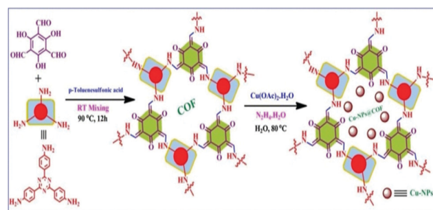
Scheme 32 The synthesis of Cu-NPs@COF. Reproduced with permission from ref. 58; copyright: 2020, Journal of CO 2 Utilization.
