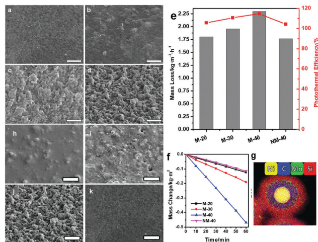
Fig. 6 SEM images of the \text{Ni}_{40}\text{C}_{20} /PVA composite film, with (a) 0 mT, (b) 100 mT, (c) 200 mT and (d) 400 mT magnetic field applied during the gelation process and the SEM images of (h) M-20, (i) M-30, (j) M-40 and (k) NM-40 (scale bar = 50 \mu\text{m} ). (e) The evaporation rates and energy conversion efficiencies of different films. (f) Water mass changes over time without light illumination at 20 ^{\circ}\text{C} on various films. (g) EDS mapping image of \text{Ni@RF@SiO}_2 core-shell nanoparticles. Reproduced with permission. 159 Copyright 2021, John Wiley and Sons.
