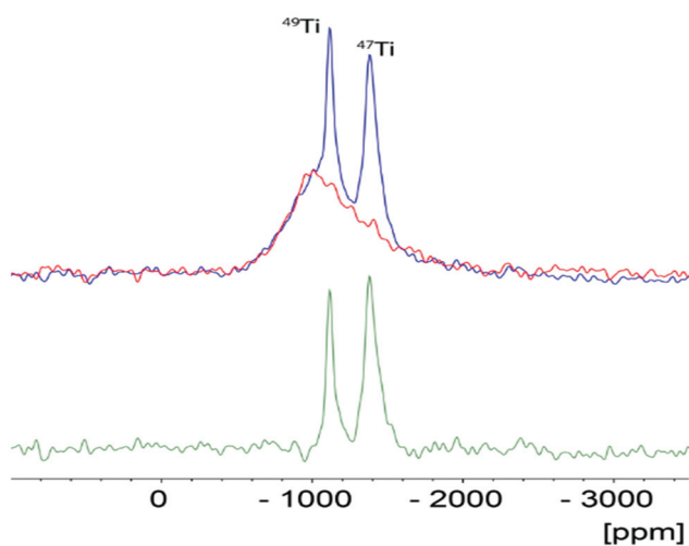
Fig. 9 Static titanium NMR spectra of \text{TiP1-H} (red) and \text{LTP-H} (blue), scaled to the same height, and their difference (green). The resonances from both titanium isotopes, ^{49}\text{Ti} and ^{47}\text{Ti} , are clearly resolved in the difference spectrum.
