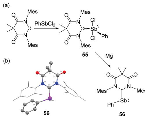
Fig. 18 (a) Syntheses of carbene-stabilized antimony adduct 55 and stibinidene 56; (b) solid-state structure of 56.
