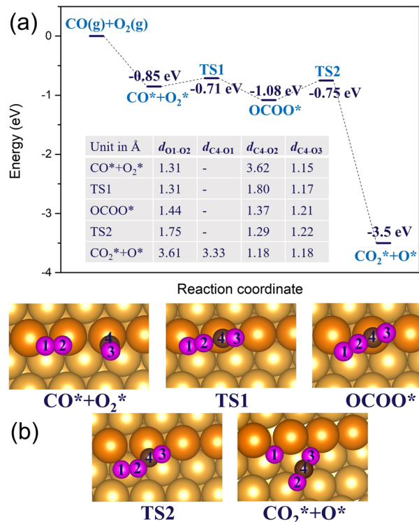
Fig. 9 (a) The reaction energy diagram and (b) the corresponding geometries of the reaction between the co-adsorbed CO* and O 2 * molecules on the regular Au(221) surface. The labelled O–O and C–O bond lengths are listed in a table embedded in the figure (a). Au atoms at the step edge are indicated by an orange color; the remaining Au atoms are shown in gold. O and C atoms of the adsorbates are shown in pink and black, respectively.
