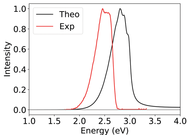
Fig. 9 Computed phosphorescence spectrum of 2CzPN obtained by employing Silver DLPNO-CCSD(T) \Delta E (black curve) and experimental phosphorescence spectrum (red curve) recorded by Hosokai et al. See text for details. 113
