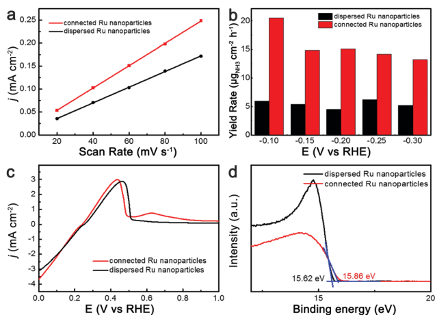
Fig. 4 (a) The differences of current density as a function of scan rate over dispersed Ru nanoparticles and connected Ru nanoparticles. (b) Normalized yield rate of NH 3 production at different potentials over dispersed Ru nanoparticles and connected Ru nanoparticles. (c) Cu-UPD stripping curves over dispersed Ru nanoparticles and connected Ru nanoparticles. (d) UPS spectra of dispersed Ru nanoparticles and connected Ru nanoparticles.
