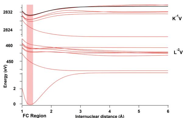
Fig. 5 Calculated potential energy curves for the ground state, the intermediate Cl K^{-1}V core-hole states and Cl L_{2,3}^{-2}(1D)V double core-hole final states. The potential energy curve of the K^{-1} ionic state is represented in black. The Franck–Condon region is indicated by the shaded vertical region.
