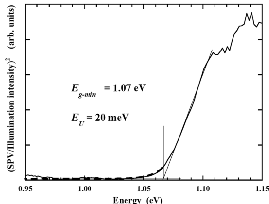
Fig. 22 Relationship between the square of the illumination intensity normalized surface photovoltage (SPV) of the CdS/CIGSSe structure and the photon energy. E_{g-\text{min}} and E_U are the minimum of the band gap energy and the Urbach energy of the CIGSSe absorber, respectively. SPV was measured in situ using a photo-assisted UHV Kelvin probe force microscope. The dashed fit line results from a fit of the subband gap SPV using the Urbach tails.
