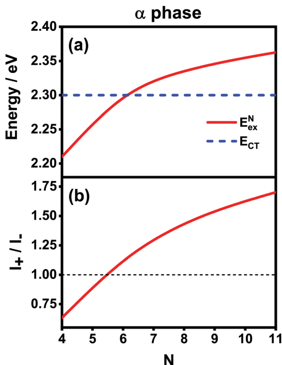
Fig. 6 Analytical results of (a) energies of the FE and CT states and (b) the intensity ratio I_+ / I_- with respect to the aggregation length for the \alpha -phase aggregates. The thin black dashed line in (b) is used to mark the position 1.00 for comparison purposes.
