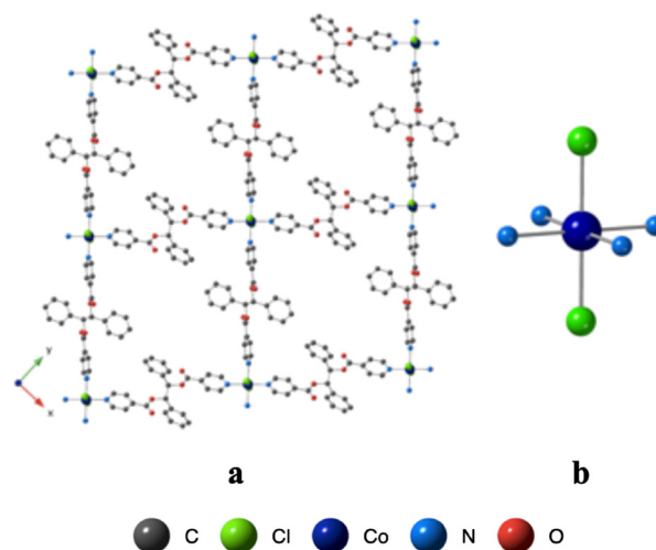
Fig. 7 Portions of the X-ray structure of L\text{-CoCl}_2 showing the formation of grids between the connection of L with \text{CoCl}_2 metallaligands (a) and environment around the \text{Co}^{2+} cations (b). H atoms and chloroform solvent are not represented for clarity.
