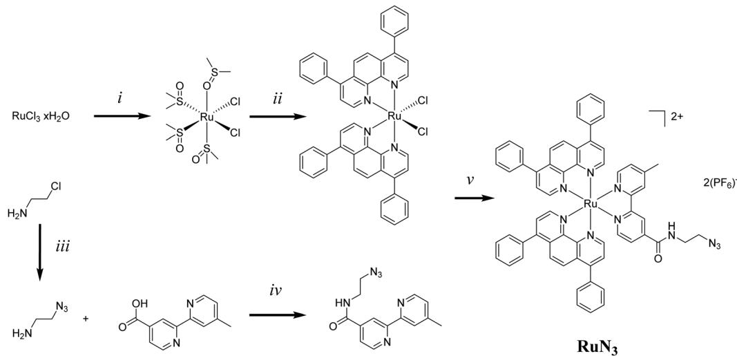
Fig. 2 Synthetic procedure for RuN 3 ; (i) EtOH/DMSO, reflux, 4 h; (ii) DMSO, 125 °C, 1 h, 85%; (iii) NaN 3 , H 2 O, 80 °C, 12 h, 82%; (iv) EDCl, NHS, DIPEA, CH 2 Cl 2 , r.t., 12 h, 56%; (v) MeOH, H 2 O, reflux, 15 h, 64%.
