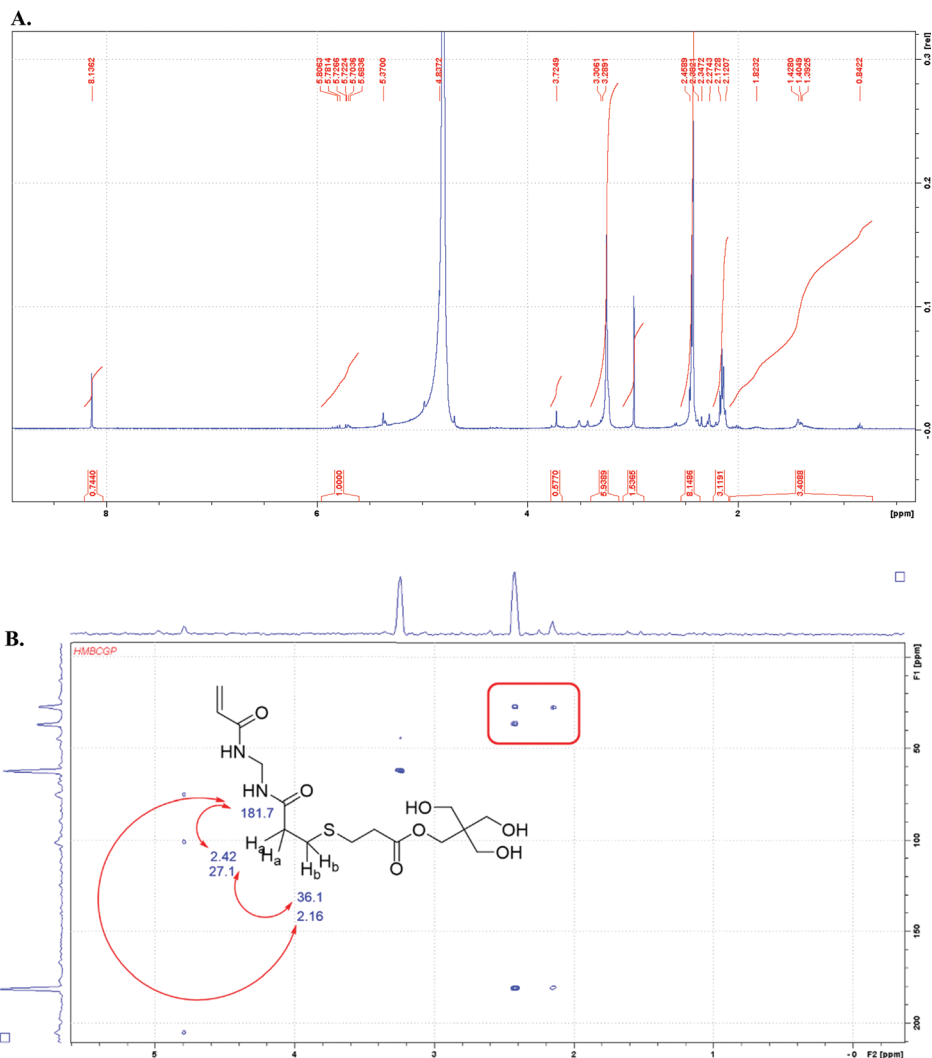
Fig. 2 The NMR analysis for 1:1 (thiol:ene) gel after basic degradation with sodium hydroxide in deuterium oxide solvent (D 2 O, 400 MHz): (A) the 1 H NMR spectrum of the hydrolysis product; (B) the gHMBC spectrum for the hydrolysis product with key correlations highlighted.
