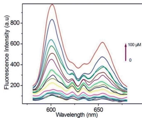
Fig. 14 Fluorescence spectra of porphyrin ligand ( 10 \text{ }\mu\text{M} ) in BBS buffer (pH = 7.40, 20 mM) after titration with \text{HS}^- from 0–100 \mu\text{M} , \lambda_{\text{ex}} = 419 . Reprinted with permission from ref. 94. Copyright (2014) American Chemical Society.
