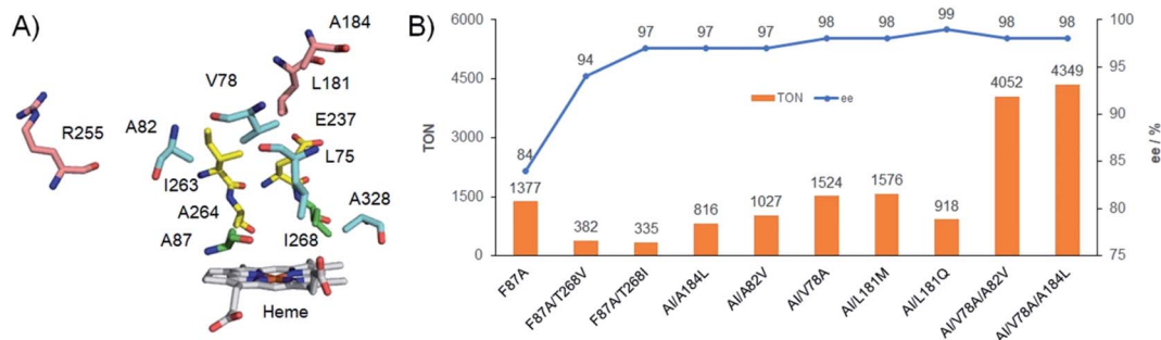
Fig. 3 (A) The residues around the active site of P450BM3 (PDB no. 1JPZ), and the residues F87 and T268 were mutated to A87 and I268, respectively. (B) Protein engineering of P450BM3 for styrene epoxidation. Experiments were performed using P450BM3 variants ( \mu M), 4 mM styrene, 20 mM (or 80 mM) H 2 O 2 , and 2 mM Im-C6-Phe in pH 8.0 phosphate buffer at 4 °C (or 25 °C) for 30 min. "AI" denoted the double mutant F87A/T268I. *In some cases, trace amounts of phenyl acetaldehydes were detected by GC.
