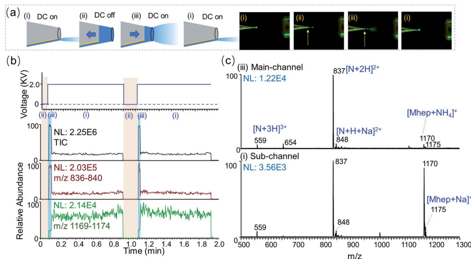
Fig. 2 Alternation between sub-channel and main-channel regimes. A solution of 10 \mu\text{M} maltotriose (Mhep) and neurotensin (N) was analyzed. (a) Left: schemes showing electrospray from the sub-channel and the main-channel, respectively. The arrows indicate the solution being accumulated or consumed. Right: photos of emitter tip in front of the MS inlet. ESI plume of the main-channel regime was visible. The dashed arrows indicate the liquid–air boundary of the accumulated solution. (b) The DC voltage applied to the pusher electrode and the corresponding ion chromatograms for total ion count, neurotensin, and maltotriose, respectively. (c) Mass spectra obtained in the main-channel ( 6.1 \text{ nL min}^{-1} ) and sub-channel ( 530 \text{ pL min}^{-1} ) regimes.
