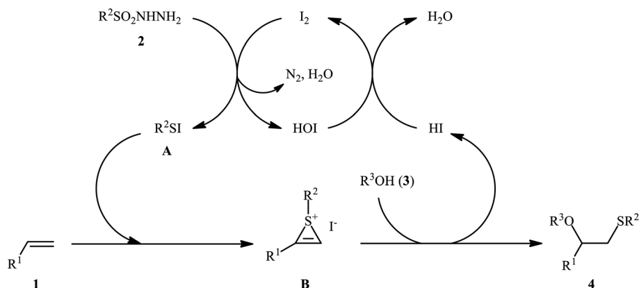
Scheme 2 \text{I}_2 -catalyzed alkoxylation of alkenes 1 with sulfonamide hydrazides 2 and alcohols 3 .
