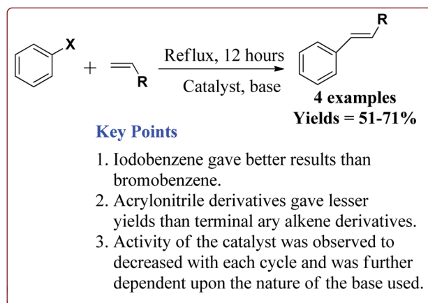
Scheme 15 Pd/( \text{SiO}_2/\text{Fe}_3\text{O}_4 ) catalyzed Heck reaction.
