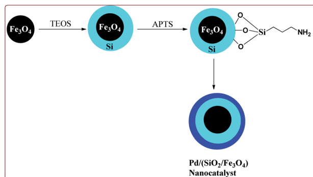
Scheme 14 Synthesis of Pd/( \text{SiO}_2/\text{Fe}_3\text{O}_4 ) nanocatalyst.
