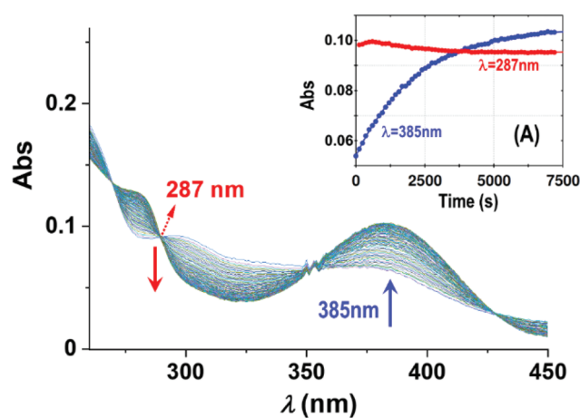
Fig. 6 Absorbance changes of 1\text{-OH}_2 (16 \mu\text{M} ) around the isosbestic point (287 nm) with time in the presence of PPI (10 equiv.; 0.16 mM) at pH 7.35 ([Tris buffer] = 10 mM) and 12 ^{\circ}\text{C} illustrating the presence of earlier reactions. Inset (A): L.S. fits of Abs vs. time at 287 nm (red) and 385 nm (blue), respectively, showing the small absorbance changes of the first reactions (induction period) and underlining the small absorbance changes therewith, not influencing the individual fits and kinetic data as illustrated in the k_{\text{obs}} vs. [\text{PPI}]_{\text{tot}} graph in Fig. 3 and 5.
