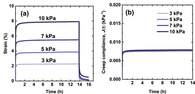
Fig. 4 Curves for the XLPHEMA-5 network showing (a) creep and creep recovery and (b) creep compliance ( J(t) = \epsilon(t)/\sigma ) at 70 °C.
