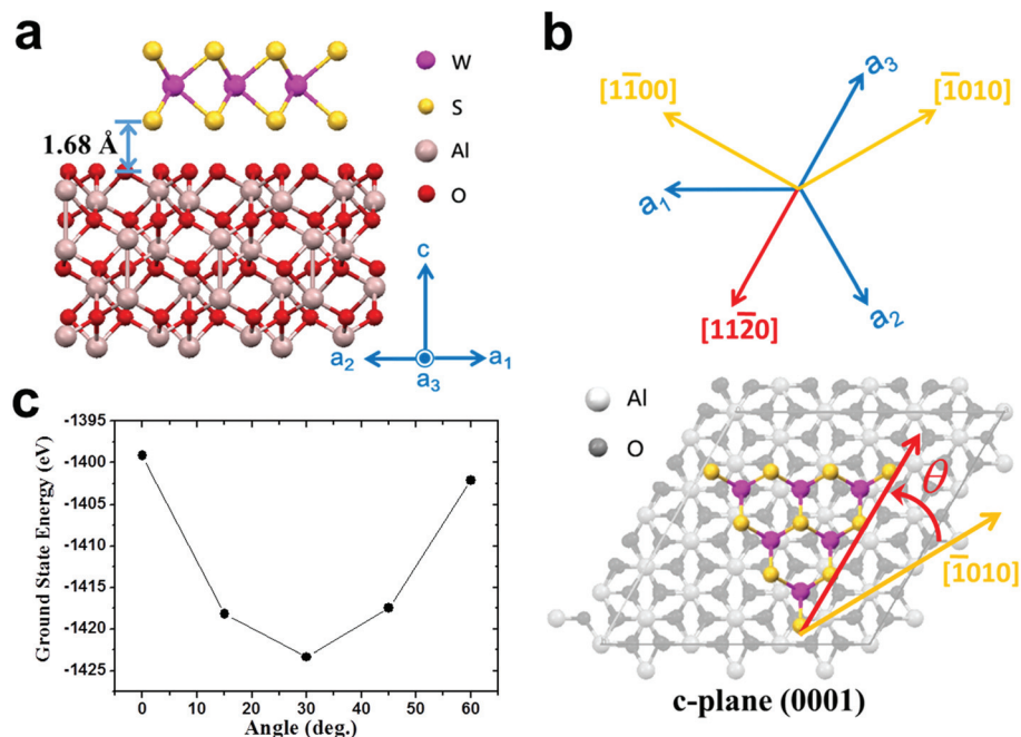
Fig. 6 First-principles DFT calculations of the optimal geometric structure and ground state energy. (a) Atomic model of the DFT calculation. Our calculation results show that the distance between NaCl-assisted WS 2 and sapphire is 1.68 Å. (b) Top view of the atomic model and the definition of the angle \theta between NaCl-assisted WS 2 and sapphire. The coordinate axis of the system is also shown. (c) Calculated ground state energy as a function of the angle between NaCl-assisted WS 2 and sapphire.
