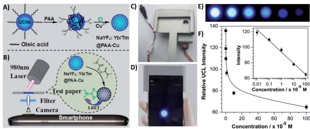
Fig. 28 Paper UCNP-based "turn-off" sensor for thiram detection. (A) Schematic illustration of the preparation procedure of NaYF 4 :Yb/Tm@PAA-Cu nanoparticles. (B) The inner optical structure of the system and the detection principle for thiram. (C) Picture of the optical attachment. (D) Frontal view of the smartphone detection setup. (E) The luminescent images of the test paper upon addition of different amounts of thiram, which were taken using the smartphone detection setup. (F) The relative luminescence intensities of color images calculated through the blue channel. The inset figure shows the linear relationship of mean luminescence intensities with the logarithm of thiram concentrations. Reprinted with permission from ref. 90. Copyright 2015, Elsevier B.V.
