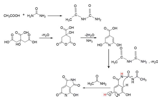
Scheme 1 The proposed mechanism of HPPT formation in the presence of AA during the synthesis process.
