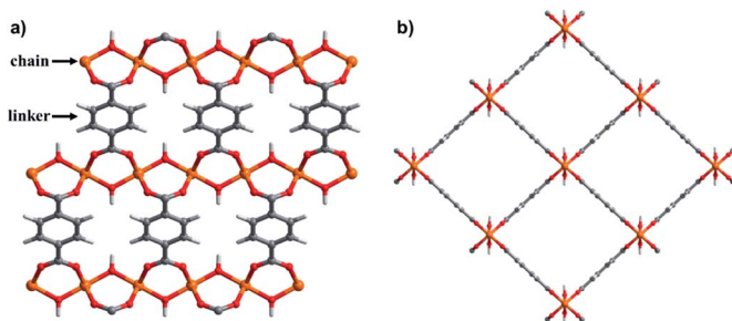
Fig. 5 Crystal structures of MIL-53(M): (a) \text{MO}_4(\text{OH})_2 chains connected by bdc linkers; (b) 1D rhombic channels in the open phase, guest molecules are omitted for clarity. Orange: M (Cr, Al, Fe, etc.), red: O, grey: C, light grey: H.
