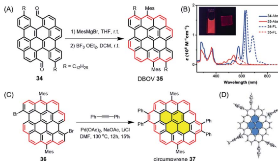
Fig. 5 (A) Synthetic route to DBOV 35 . (B) UV/Vis absorption and fluorescence spectra of precursor 34 and DBOV 35 . Inset: Images of DBOV 35 in solution and 1 wt% polystyrene composite film under UV irradiation. 107 Copyright 2017. Adapted with permission from WILEY-VCH Verlag GmbH & Co. KGaA, Weinheim. (C) Synthesis of circumpyrène 37 via transition metal-catalysed benzannulation; DMF = dimethylformamide. (D) Single-crystal structure of circumpyrène 37 . 112 Copyright 2019. Adapted with permission from the American Chemical Society.
