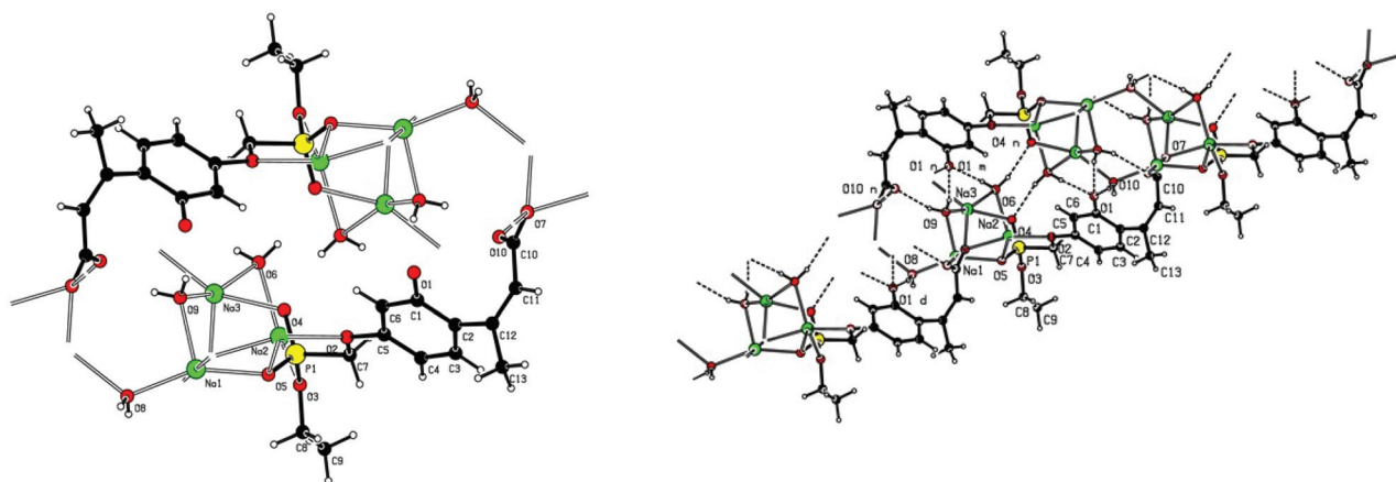
Fig. 5 X-ray structure of 2a trisodium 3-[4-(ethoxy-phosphonomethoxy)-2-phenolato]-but-2-enoate trihydrate. Left: showing \text{Na}^+-\text{O}-\text{P} , \text{Na}^+-\text{O}-\text{C} and \text{Na}^+-\text{OH}_2 bonding. Right: the extended hydrogen bonded chain structure.
