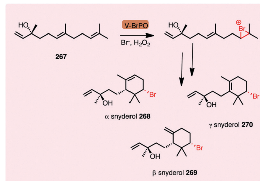
Scheme 11 V-BrPO catalysed terpene bromination and cyclisation event in snyderol biosynthesis. 184
